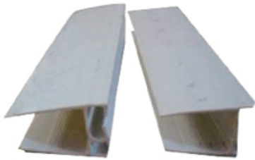
Polymer Invisible Flange/ Polymer Joint Flange (Fire Retardant Type) Length : 4 Meter Thickness : 20 mm, 30 mm Order Code : 20 INF, 30 INF
